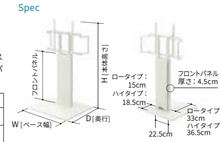
PRODUCT INFO. V5 HIGH TYPE / COLOR: SATIN WHITE / TV size: 70inch / OPTION: SOUNDBAR SHELF L size
