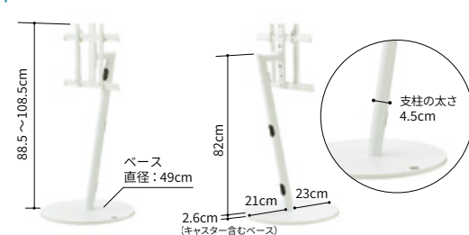
PRODUCT INFO. A2 LOW TYPE / COLOR: SATIN WHITE / TV size: 55inch
